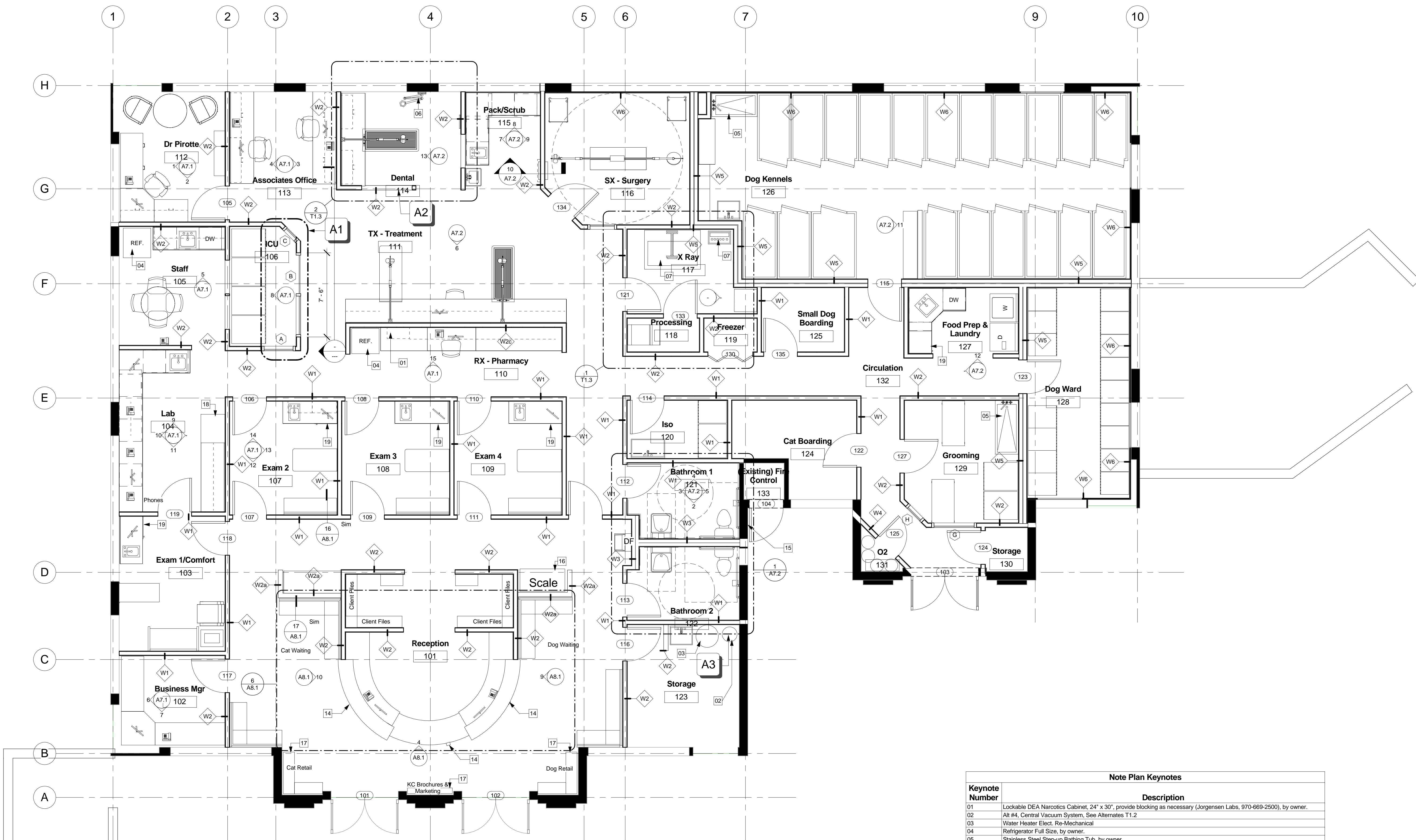
1 First Floor Note Plan A1.1 1/4" = 1'-0"
